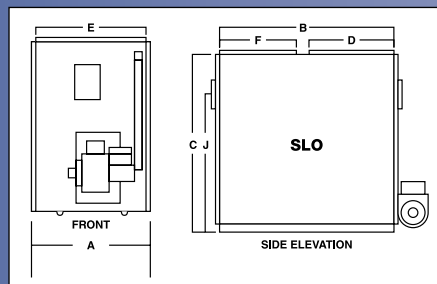
DIMENSIONS LOWBOY
